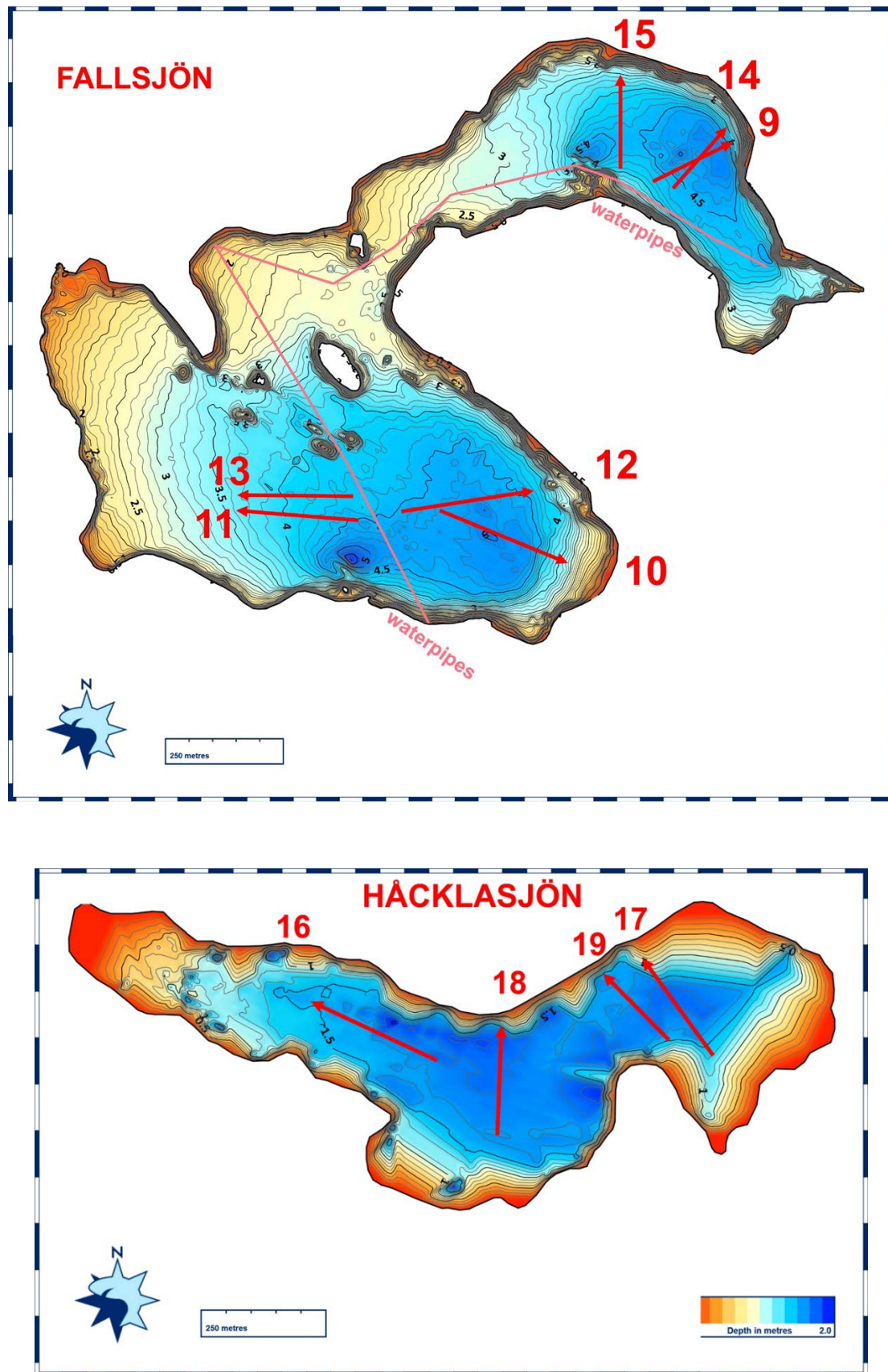
Figure 4. The locations of the hauls made in the reduction fishing of cyprinids by seining at Lake Fallsjön and at Lake Håcklasjön in autumn 2021. The layout depth map is by Husshållningssällskapet, Ola Helmersson.
